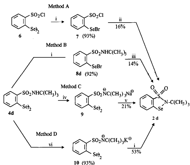
Scheme 3. (i) Br 2 , CCl 4 , -10 to 20°C. – (ii) H 2 NC(CH 3 ) 3 , CH 2 Cl 2 , -10°C. – (iii) (C 2 H 5 ) 3 N, CCl 4 , -10°C. – (iv) NaH, CH 2 Cl 2 , 20°C. – (v) Br 2 , CH 2 Cl 2 , -10 to 20°C. – (vi) t BuOK, t BuOH, reflux
